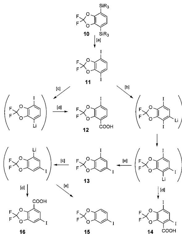
[a] 2.0 eq ICl in tetrachloromethane at reflux. [b] Lithium diisopropylamide (LIDA) in tetrahydrofuran (THF) at -75^{\circ}\text{C} . [c] Butyllithium (LiC) in tetrahydrofuran at -75^{\circ}\text{C} . [d] (1) \text{CO}_2 , (2) HCl. [e] \text{H}_3\text{COH} .
